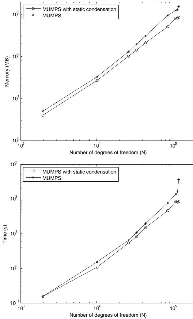
Figure 1: Memory and time savings from Static Condensation before the application of the Mumps solver.
